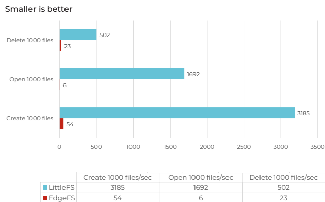
Figure 2. EdgeFS random file creation, access, and deletion superior to alternative
